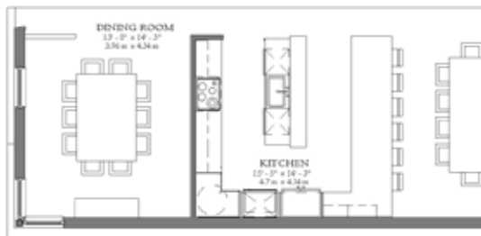
ALTERNATE KITCHEN
