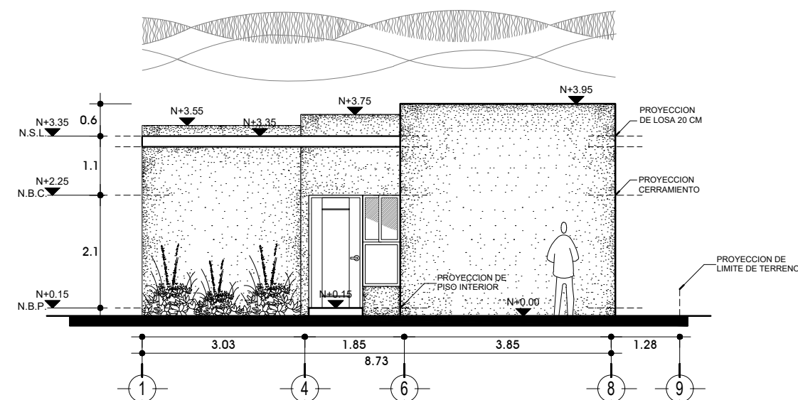
Fachada Principal
