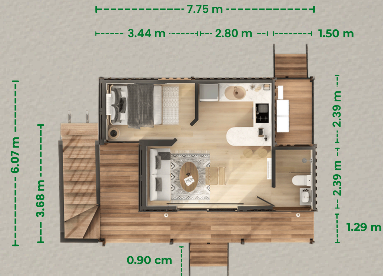
Ground Floor
