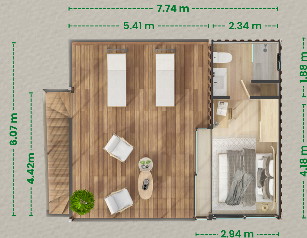
Upper Floor
