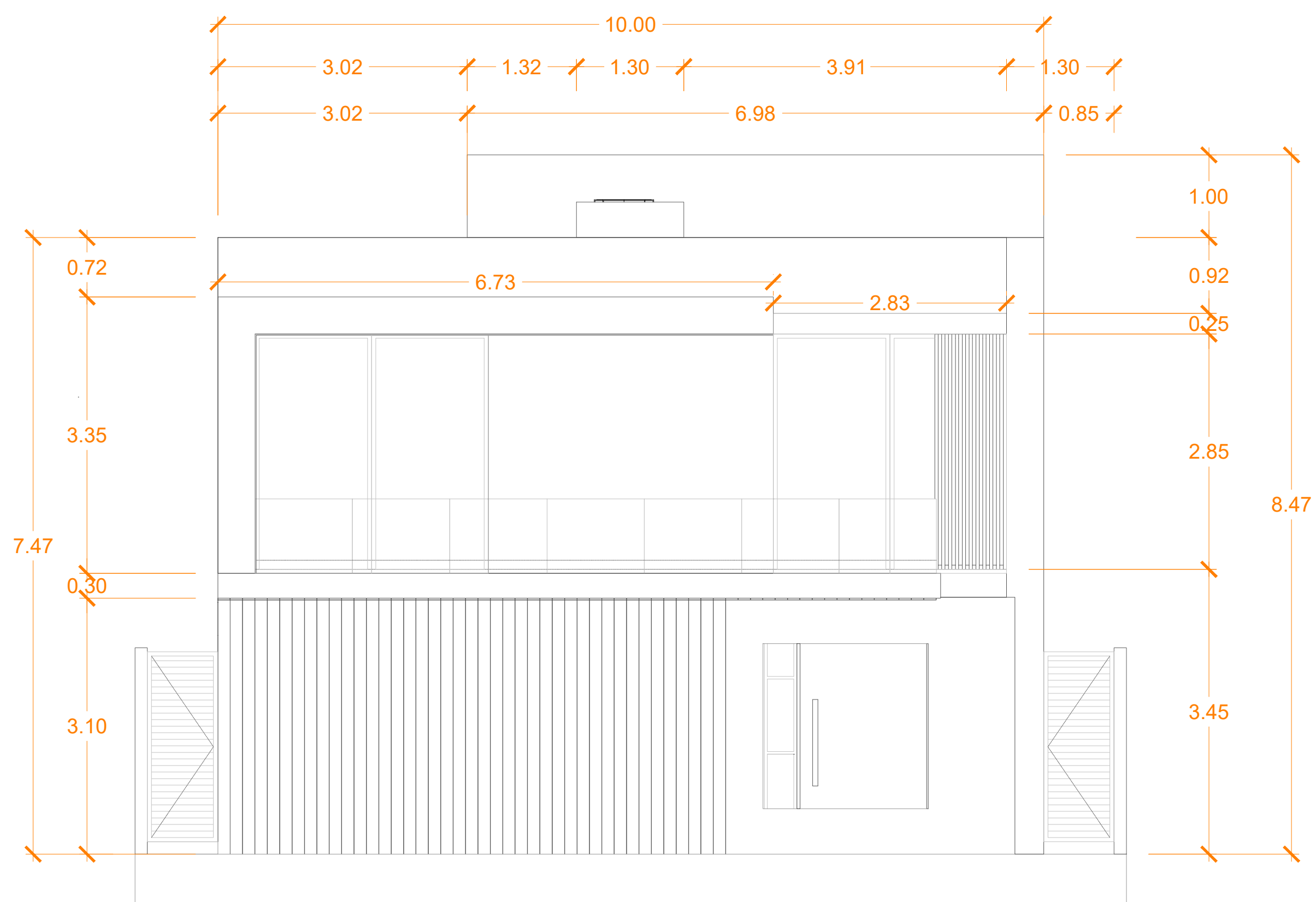
FACHADA PRINCIPAL
