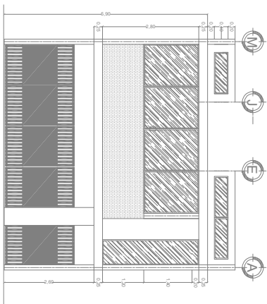
FACHADA PRINCIPAL
