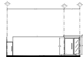
Fachada Principal ESCALA 1:100
