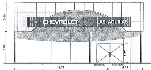
Fachada Principal
