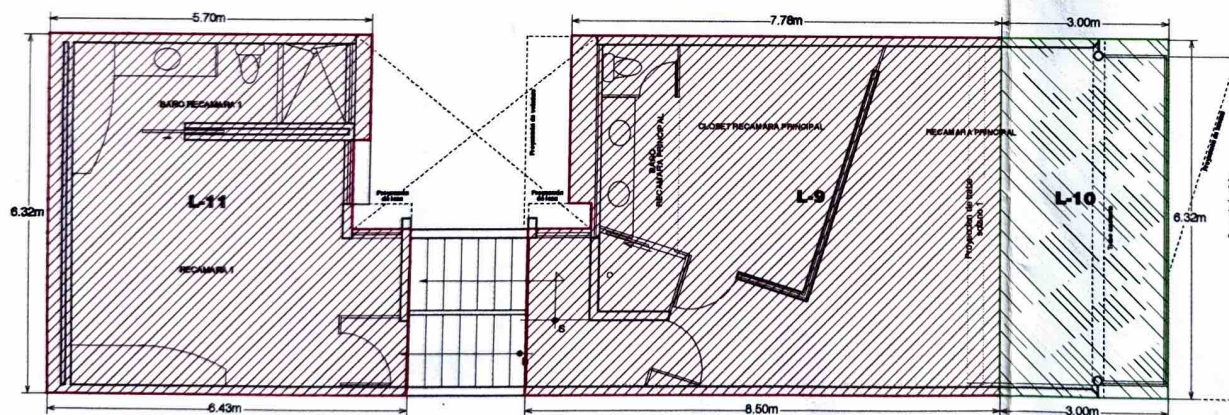
LOSA "L - 11" RECAMARA 1 (5.32 X 6.43 = 37.70 M2)
