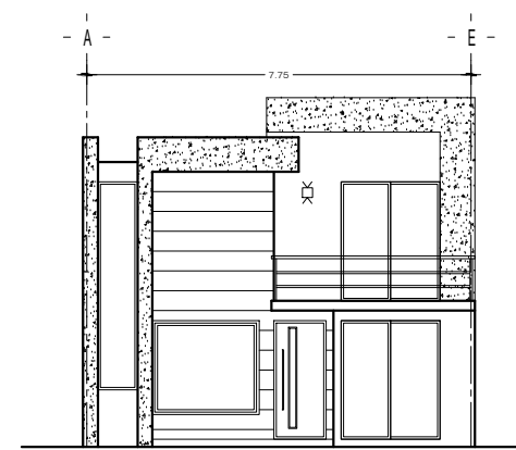
FACHADA PRINCIPAL
