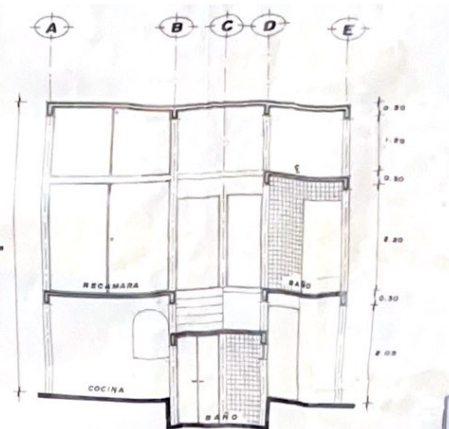
CORTE TRANSVERSAL Y-Y'
