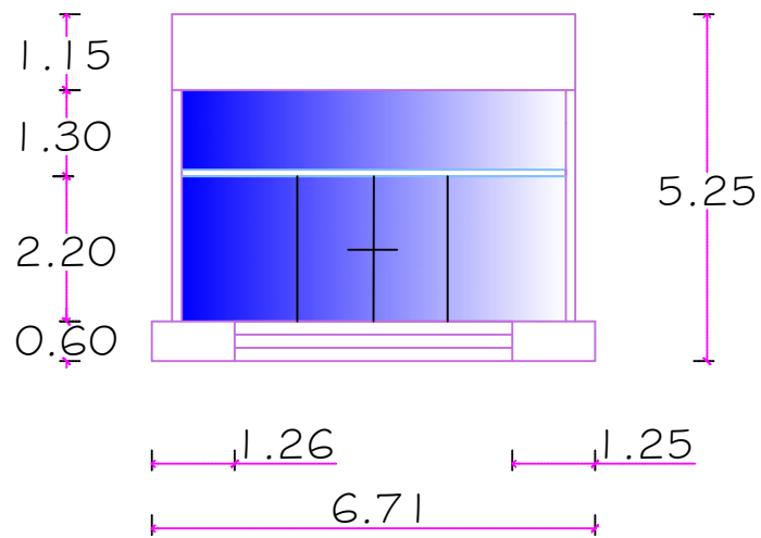
Facada frontal
