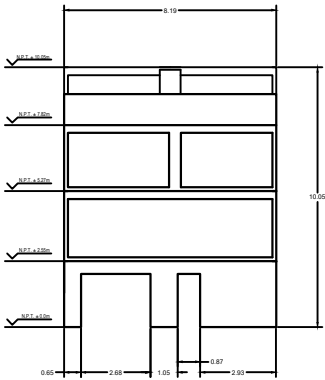
Fachada Principal
