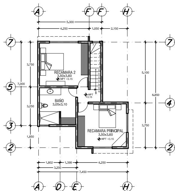
PLANTA ALTA AREA: 51.51 M2
