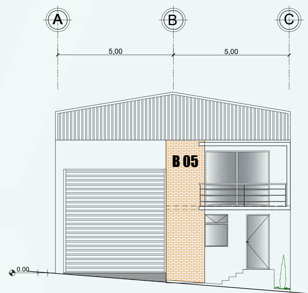
VISTA FRONTAL
