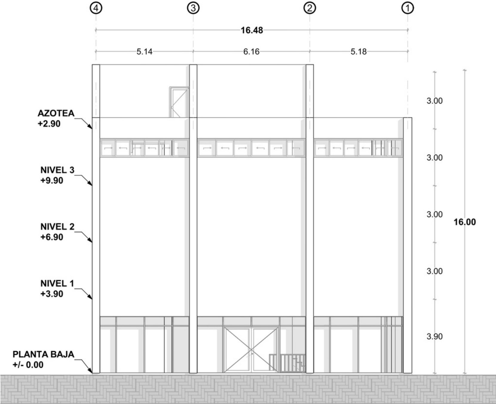
FACHADA PRINCIPAL
