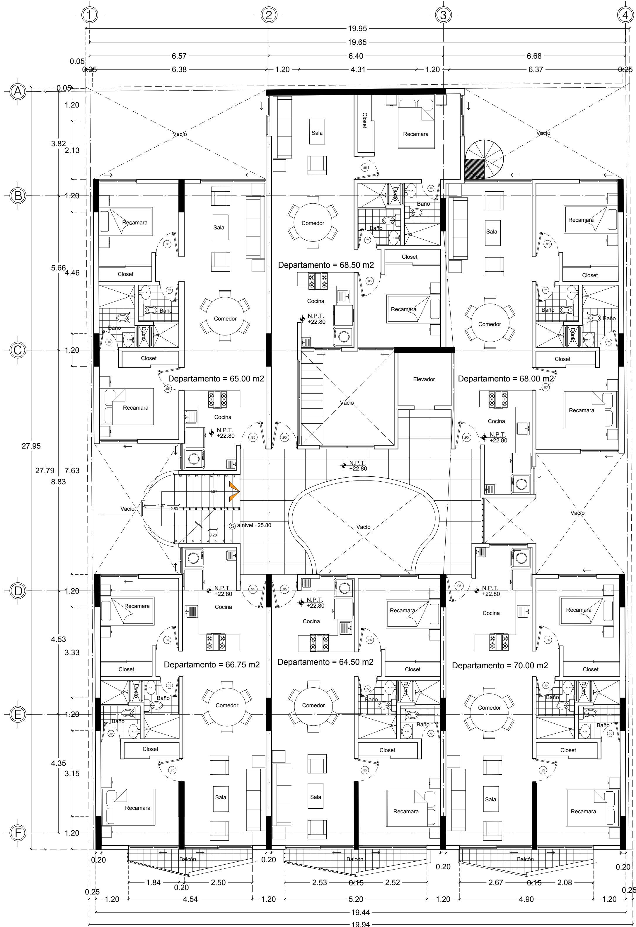
PLANTA PH'S
