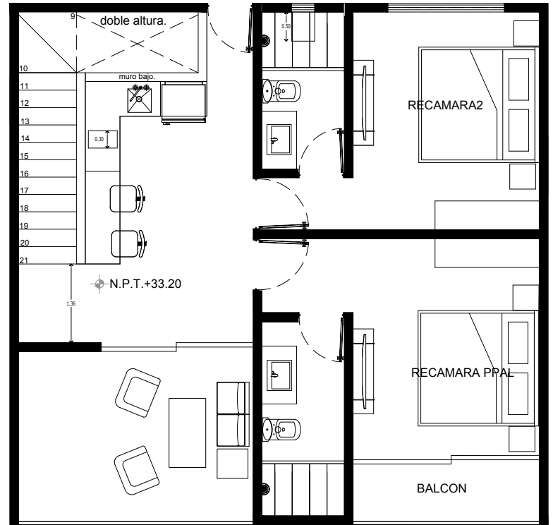
PLANTA ALTA ( LOCK OFF )
