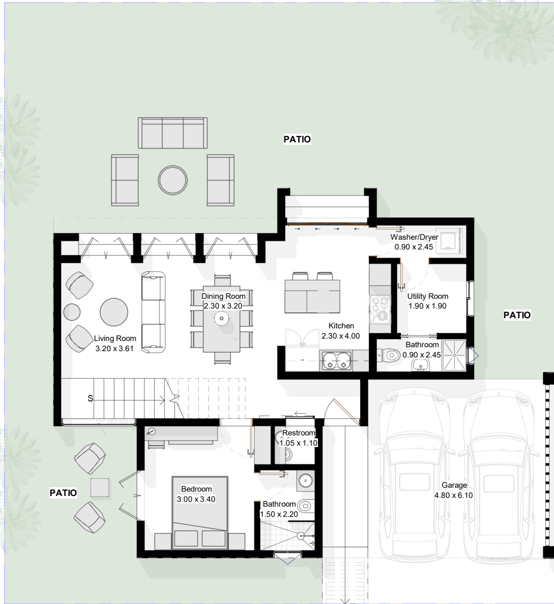
1 FIRST FLOOR LEVEL ESC: 1 : 100
