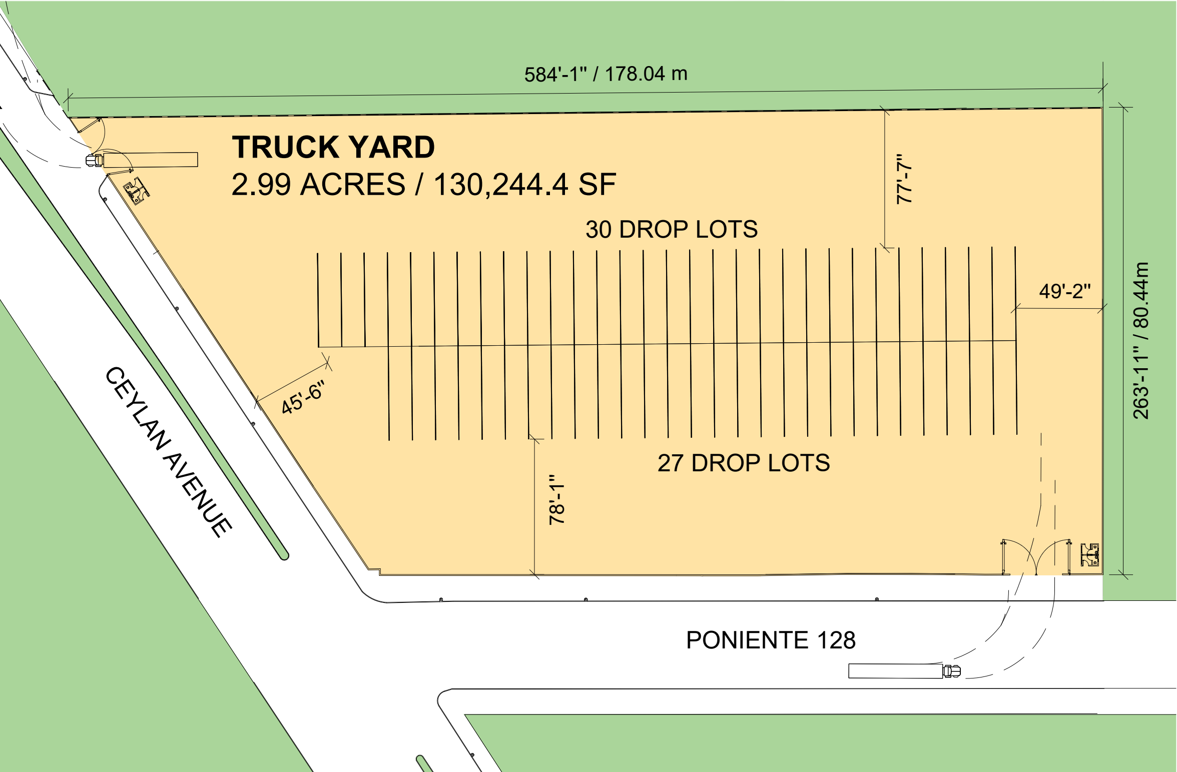
SITE PLAN
