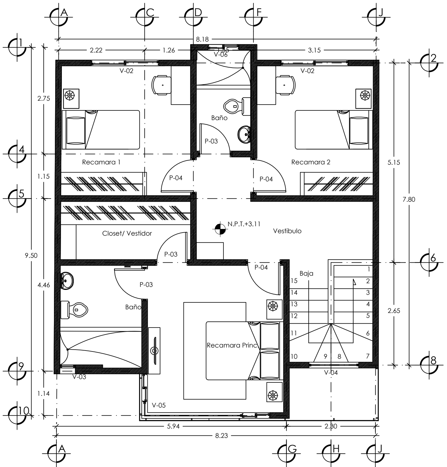
PLANTA ARQUITECTONICA ALTA AREA = 72.5m 2
