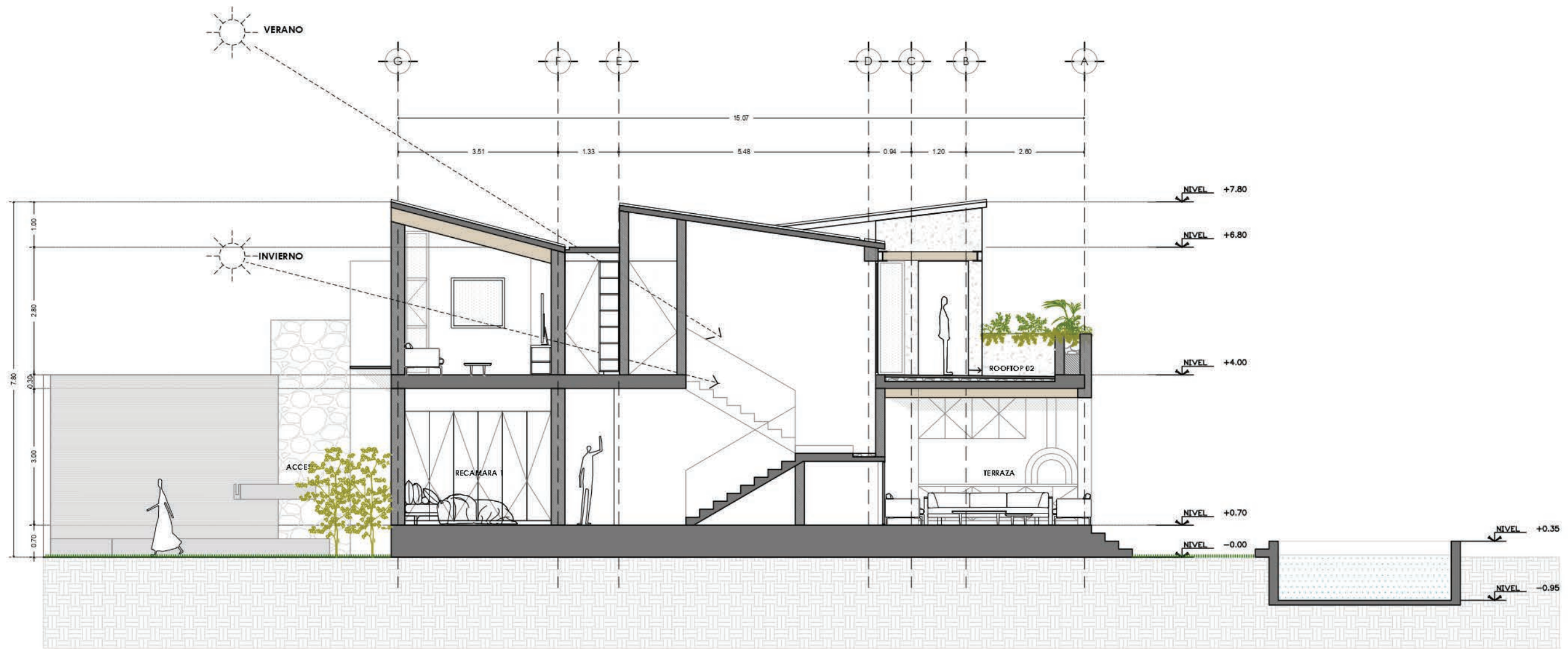
CORTE 4-4'
