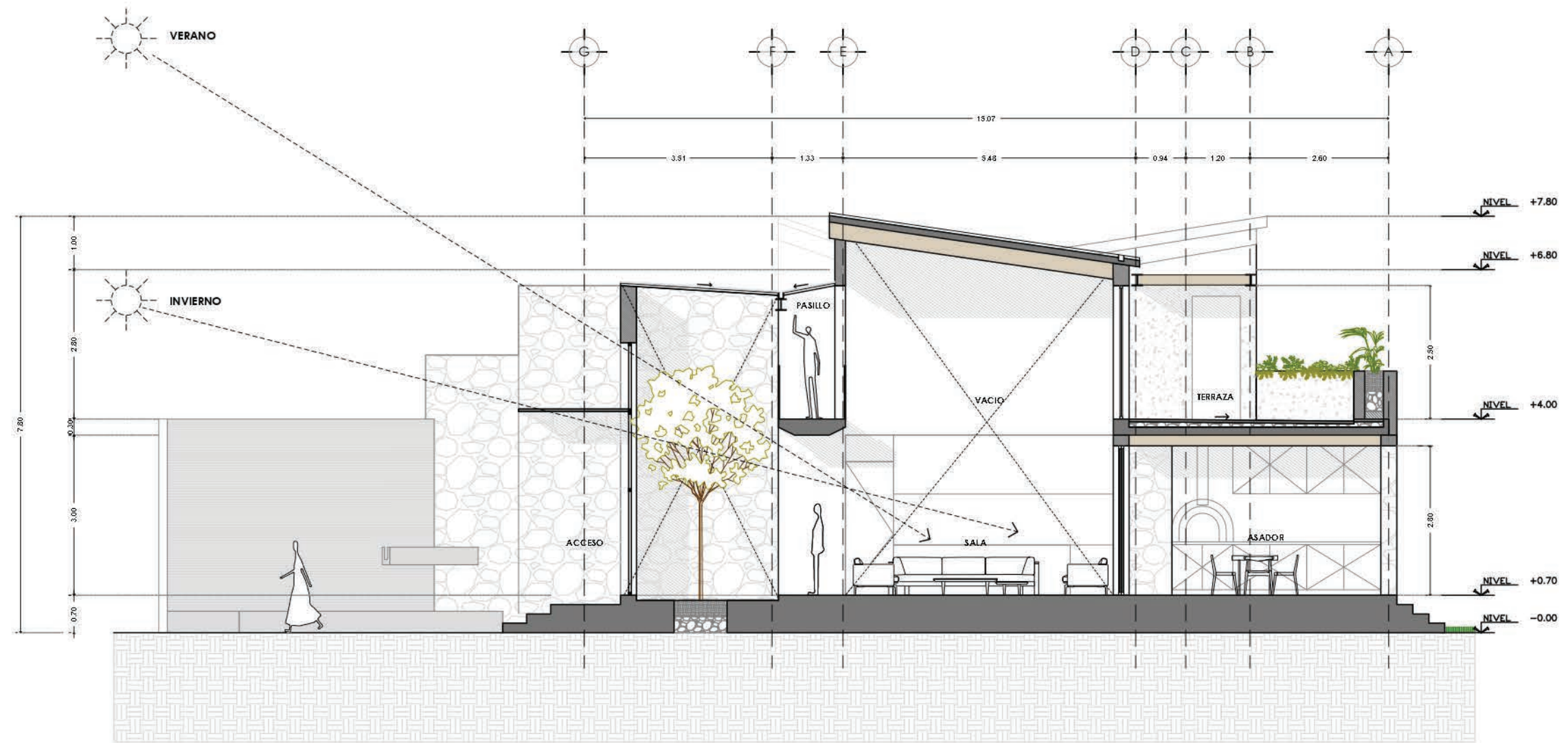
CORTE 5-5'
