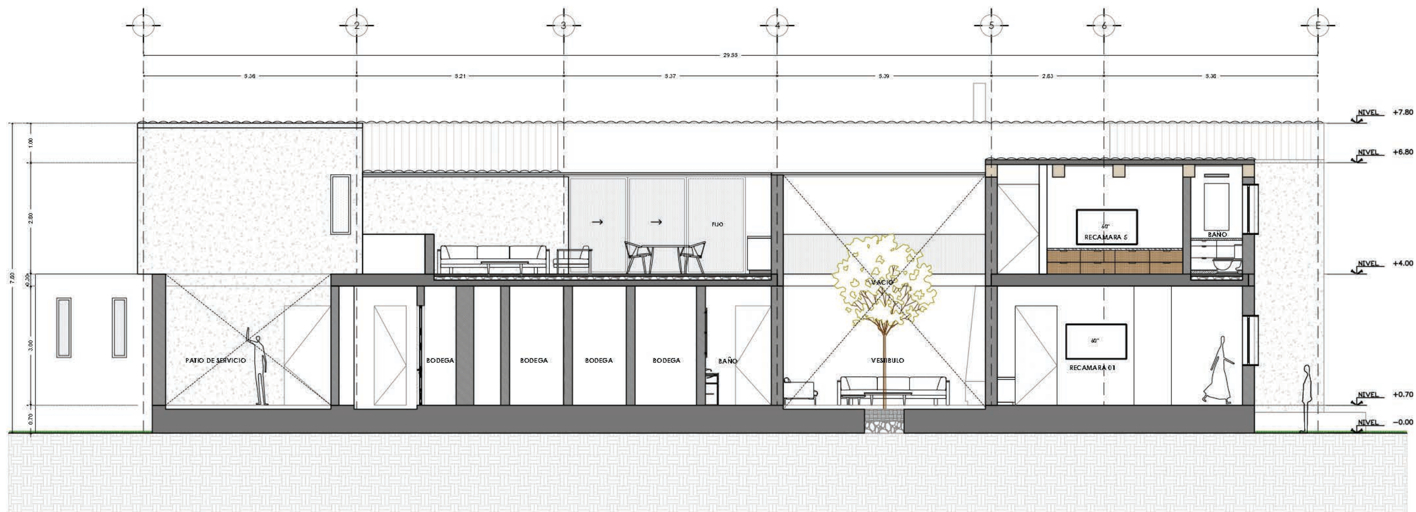
CORTE 2-2'
