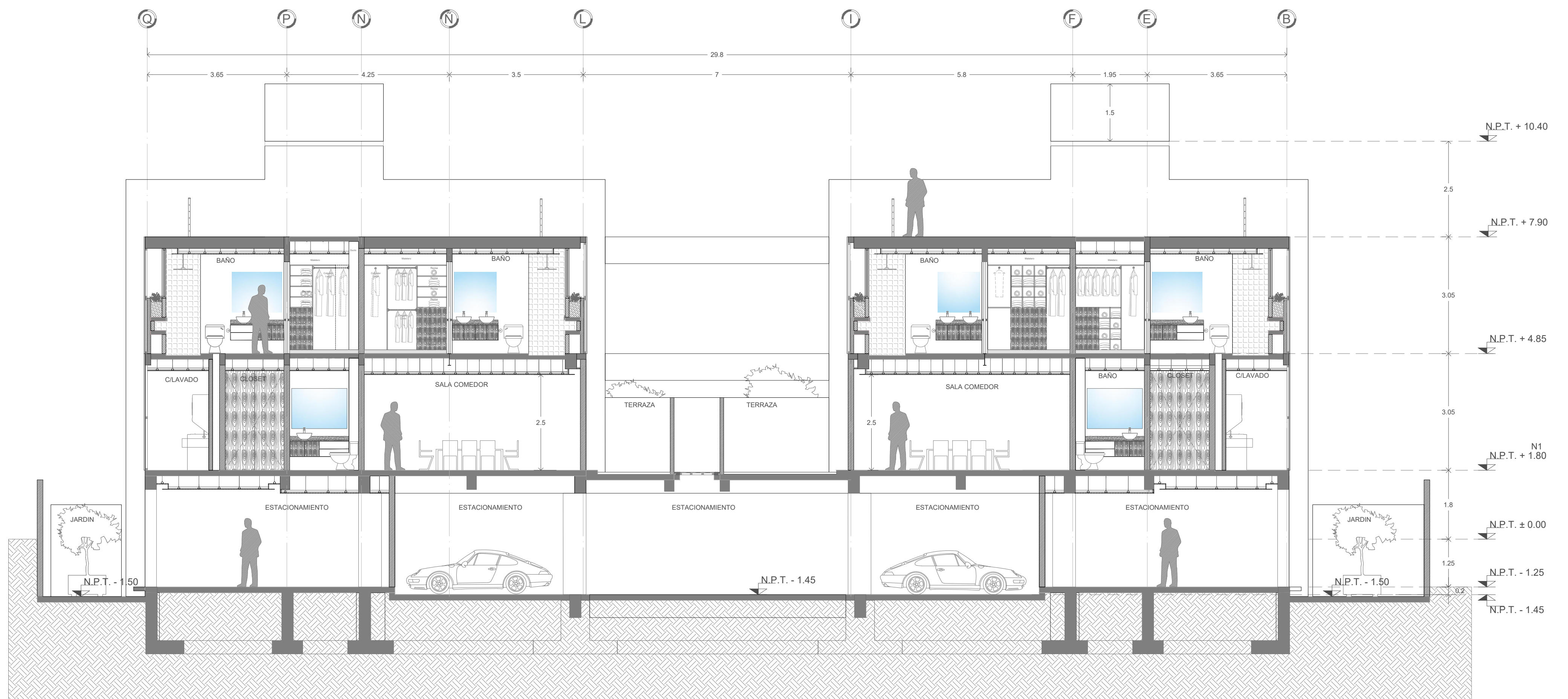
02 CORTE TRANSVERSAL H-H 1:75
