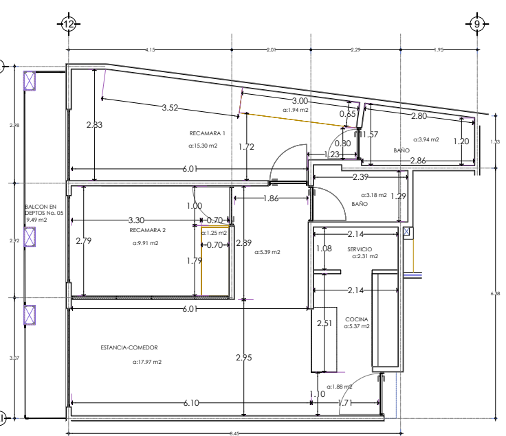
AREAS T-2R-1.4 ESC. 1:125 ACOT. M
