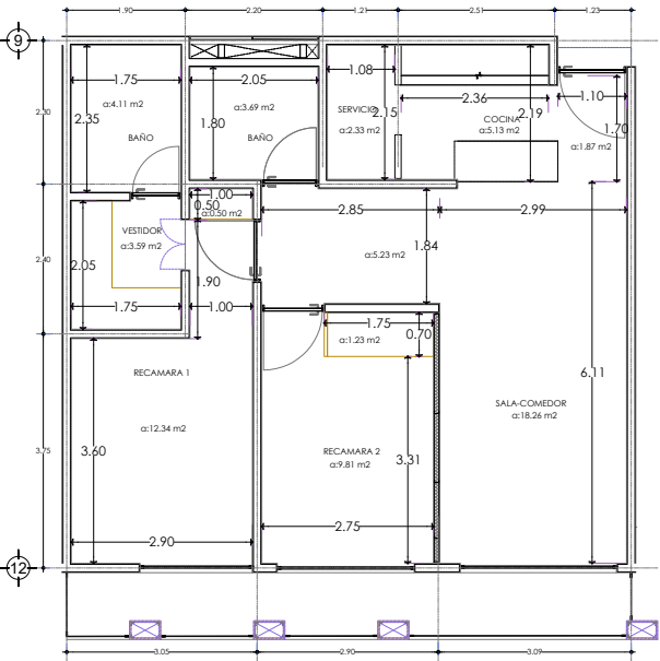
AREAS T-2R-1.3A ESC. 1:125 ACOT. M
