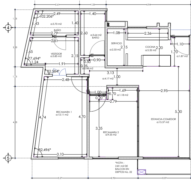
AREAS T-2R1.1 ESC. 1:125 ACOT. M
