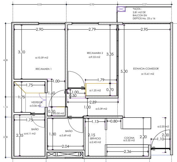
AREAS T-2R1.2 ESC. 1:125 ACOT. M
