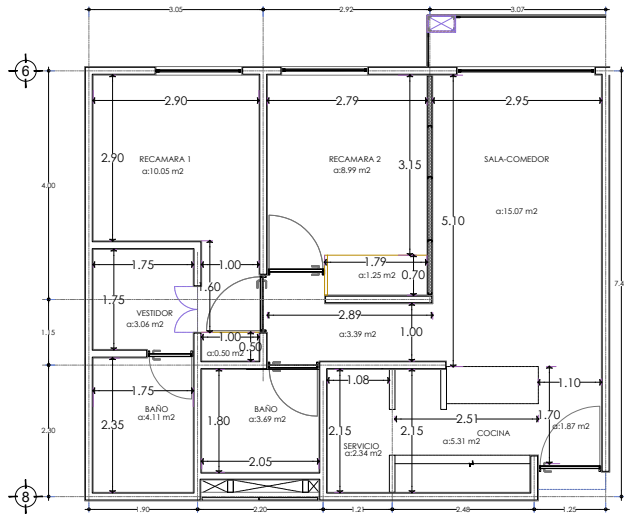
AREAS T-2R-1.3 ESC. 1:125 ACOT. M
