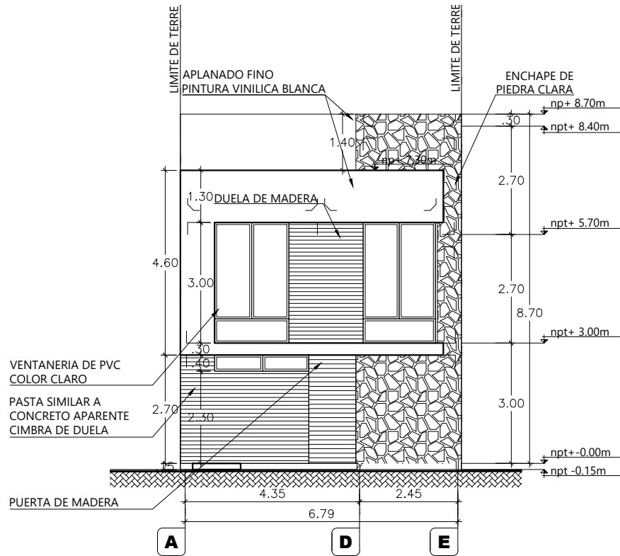
Alzado Principal
