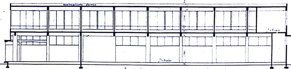
Section 1-1 ALL WINDOWS
