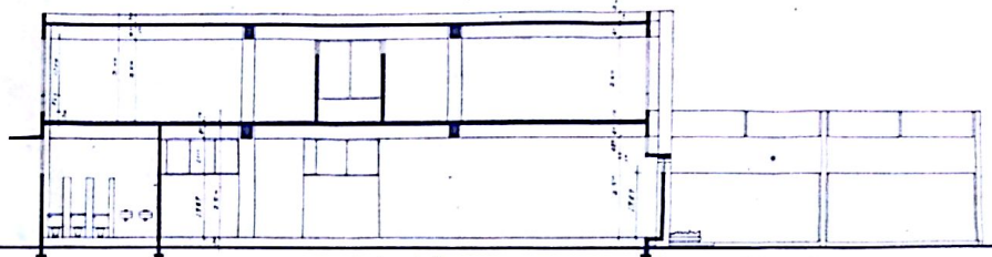
Section 2-2 ALL WINDOWS
