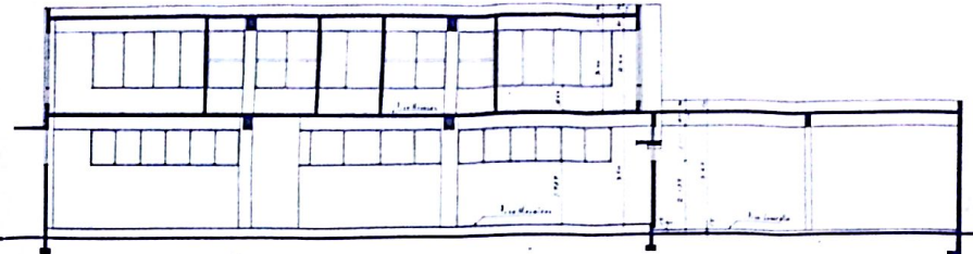
Section 3-3 ALL WINDOWS
