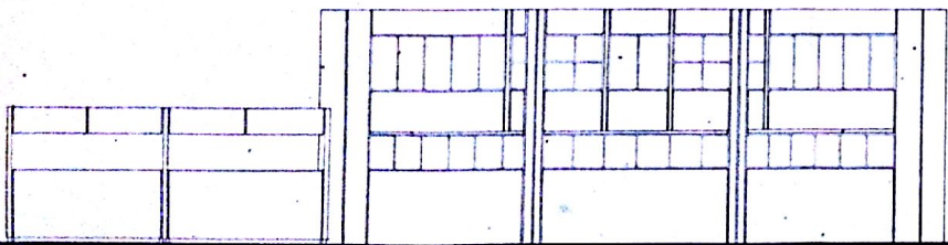
Elevation S.W. ALL WINDOWS
