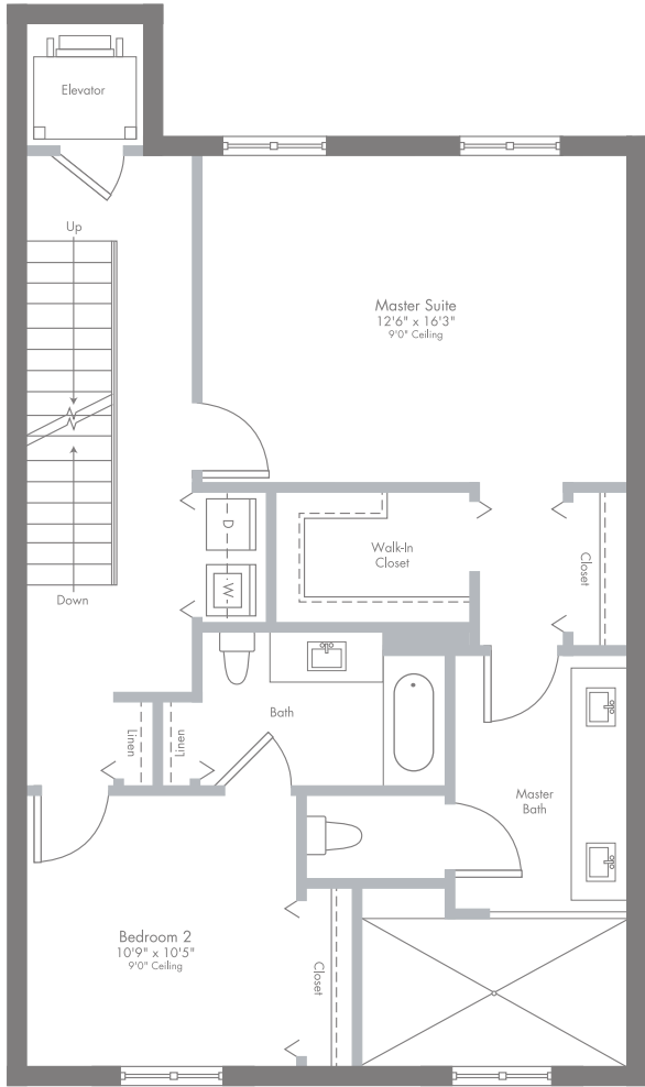
THIRD FLOOR
