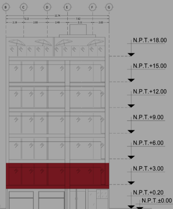
FACHADA PRINCIPAL CALLE VOSGOS LOMAS
