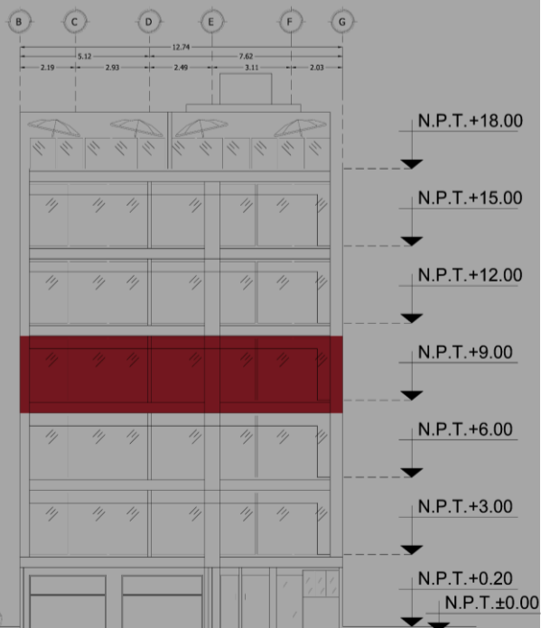
FACHADA PRINCIPAL CALLE VOSGOS LOMAS
